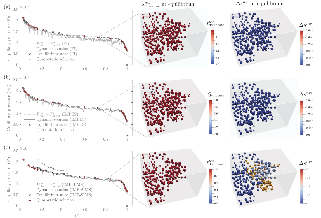
Figure 3. Comparison of equilibrium solutions between the dynamic and quasi-static simulations in Network 1: (a) FI method, (b) IMPES method, and (c) IMP-SIMS method. The pressure difference between two boundaries P_{\text{inlet}}^{nw} - P_{\text{outlet}}^{nw} (dash-dot line), dynamic interfacial-area-weighted capillary pressure P^c (solid line), and P^c at equilibrium states (dark cross) for the dynamic simulations are plotted as functions of the domain-averaged wetting phase saturation S^w using the P^c - S^w for the quasi-static simulations (red plus sign) as a reference (left column). The fluid configuration at the equilibrium state for P_{\text{inlet}}^{nw} = 13 kPa (middle column) and the corresponding pore-by-pore saturation difference between quasi-static and dynamic solutions ( \Delta s^{nw} = s_{\text{quasi-static}}^{nw} - s_{\text{dynamic}}^{nw} ) (right column) are presented for all three methods. Only the invaded pores are shown. Note that in the right column, the pore bodies that are invaded in the quasi-static simulation but not invaded in the dynamic simulation (i.e., s_{\text{dynamic}}^{nw} = 0 while s_{\text{quasi-static}}^{nw} > 0 ) are identified by orange color.
